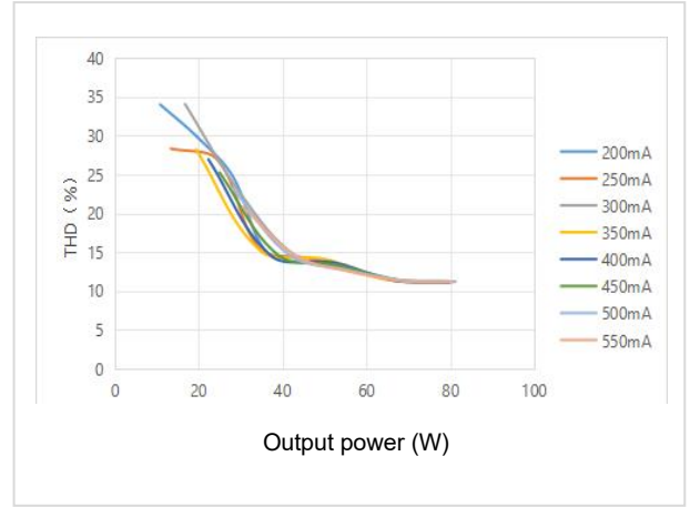
THD Curve
